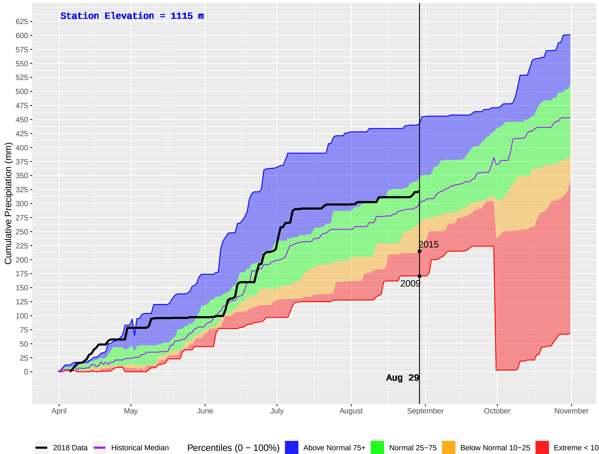
SICAMOUS (882) : Historical (2004–2016) and Current (2018) Daily Cumulative Precipitation
